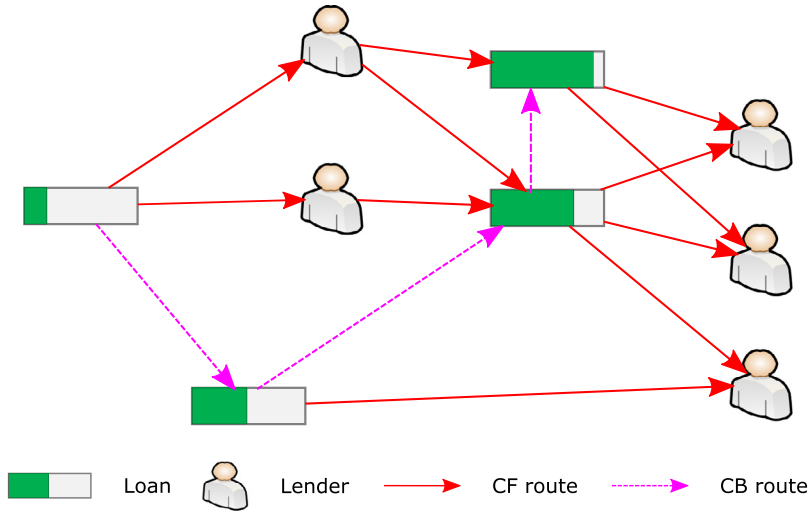
Fig. 2. Graph structure of RWH.
